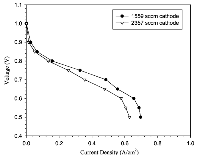
Figure 6. Bulk polarization curves for condition 2. RH = 100/0 anode/cathode.
